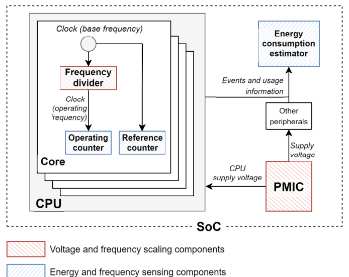
Fig. 1: A typical DVFS implementation, illustrating components used for sensing operating frequency and supply voltage.
